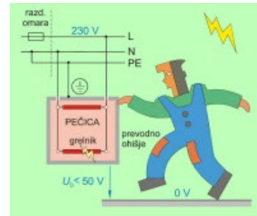
Slika 3: Posredni dotik http://eoet1.evsebina.com/material/eOet1_02_06_02-2.html
